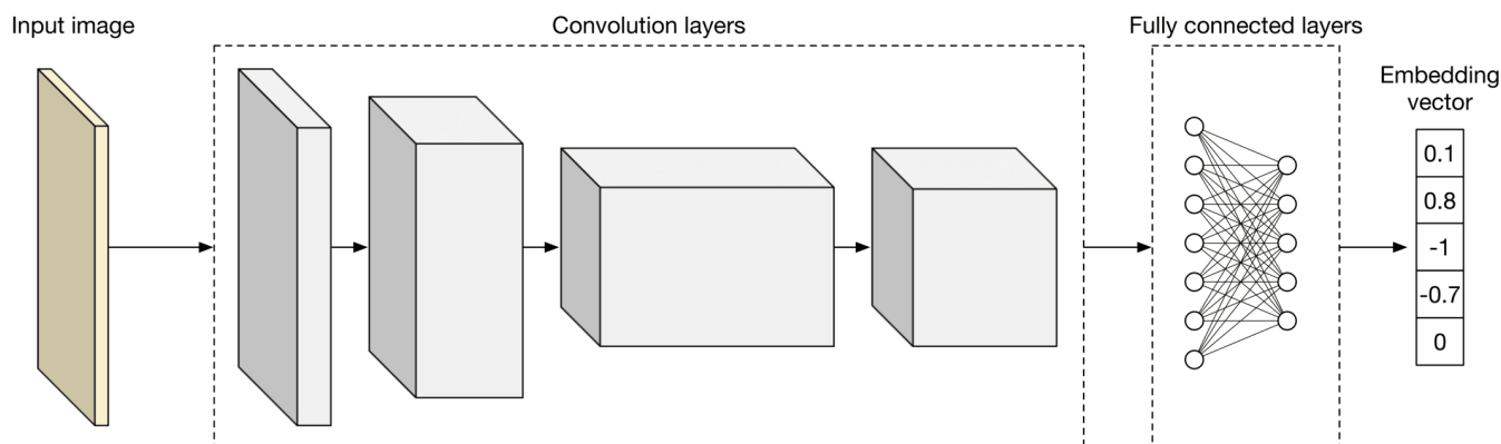
Figure 2.5: A simplified model architecture
