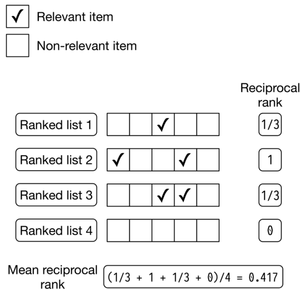
Figure 2.13: MRR calculation example
