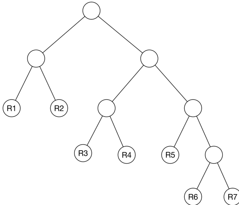
Figure 2.22: A formed tree from the points
