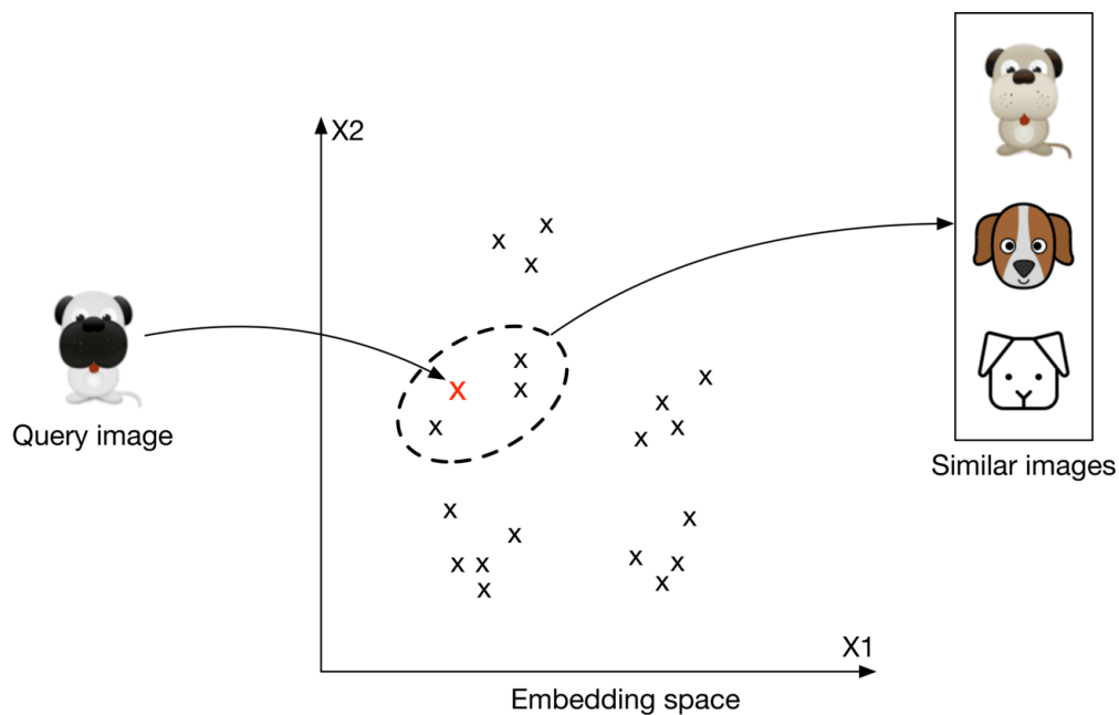
Figure 2.4: Top 3 images similar to the query image
