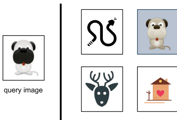
Figure 2.6: Contrastive training
