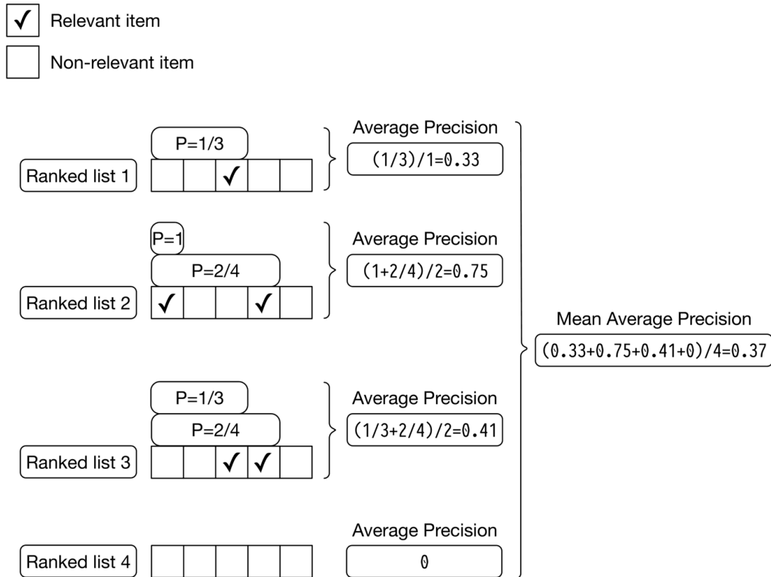
Figure 2.16: mAP calculations
