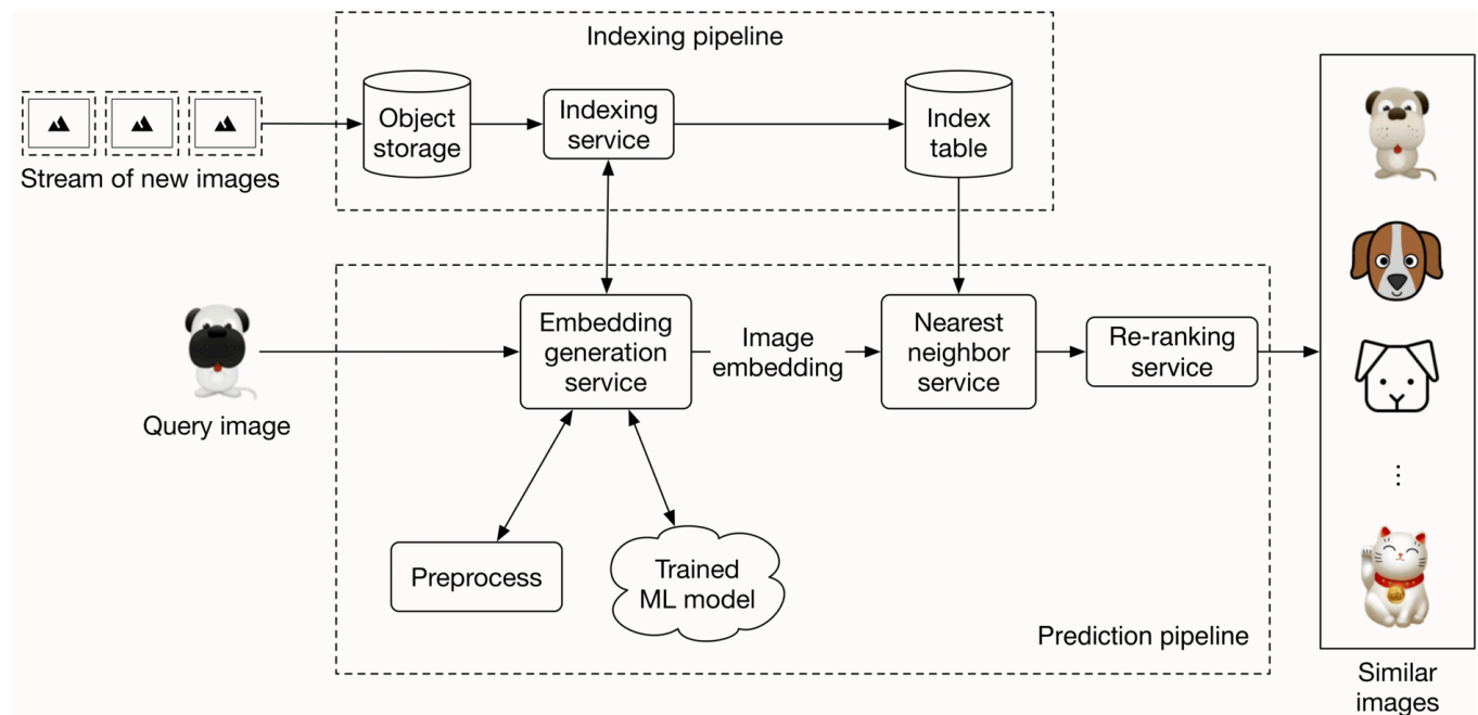
Figure 2.19: Prediction and indexing pipeline
